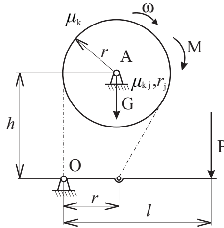
Figure 3.57: Problem 3.8.6. Equilibrium of a brake drum
