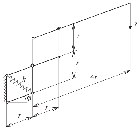
Figure 3.83: Exercise 3.12.3. Equilibrium of a mechanism
