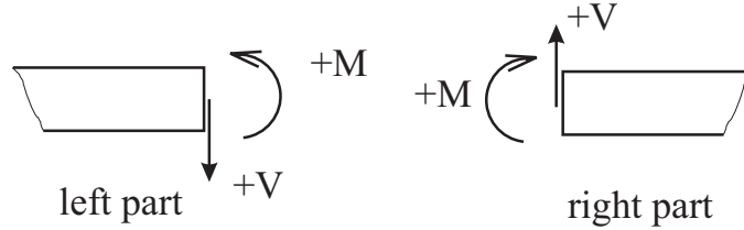
Figure 3.66: Internal forces in a beam
