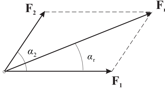
Figure 3.1: Parallelogram law.
