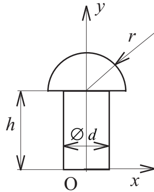
Figure 3.63: Exercise 3.9.5. The centroid of a rivet
