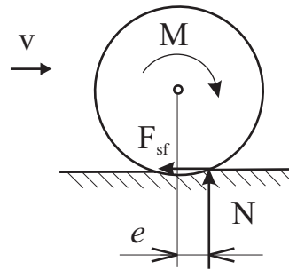
Figure 3.50: Rolling resistance
