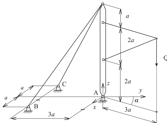
Figure 3.35: Exercise 3.5.5. Equilibrium of a rotating crane
