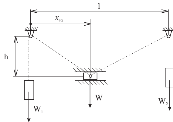
Figure 3.18: Exercise 3.3.3. Equilibrium of the weight
