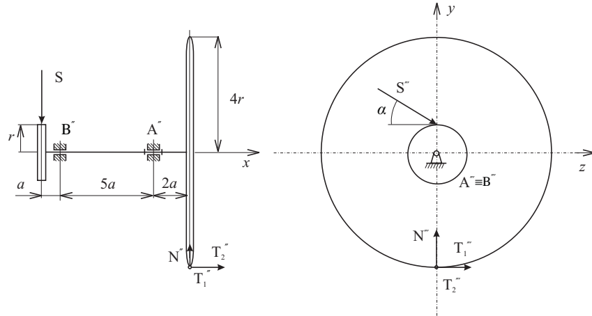
Figure 3.33: Exercise 3.5.3. Equilibrium of a semiaxle
