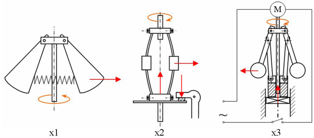
Figure 3 Illustration of redesign process – input to the CRDP system – three old solutions.
